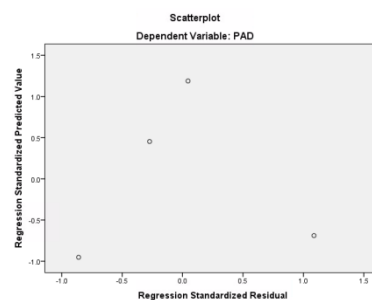
Gambar 1 : Scatterplot
